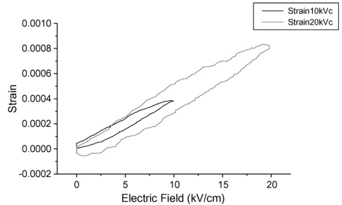
Fig. 11. Unipolar strain hysteresis measurement for (K_{0.34}Na_{0.64}Li_{0.02})(Nb_{0.96}Sb_{0.04})O_3 ceramic.
