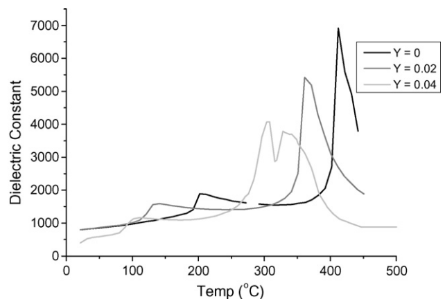
Fig. 7. Temperature dependence of dielectric constant for KNN-LS samples ( y = 0, 0.02 and 0.04 ) at 100 KHz.
