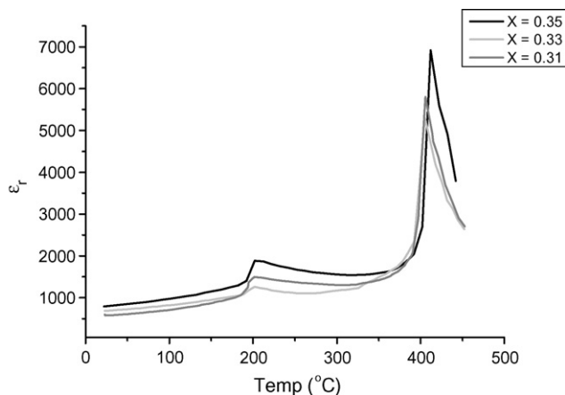
Fig. 5. Temperature dependence of dielectric constant for KNN samples ( x = 0.35, 0.33 and 0.31 ) at 100 KHz.
