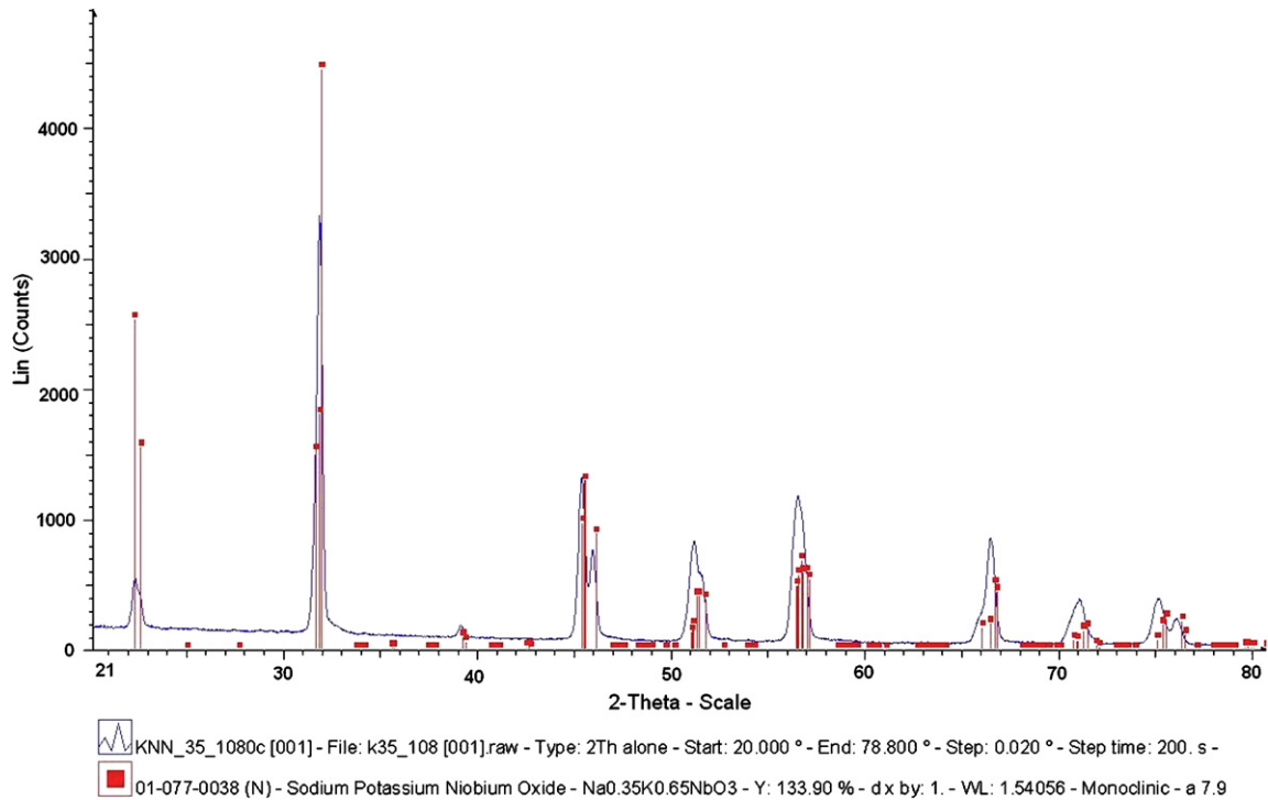
Fig. 4. XRD patterns of K_{0.35}Na_{0.65}NbO_3 fitted with reference plot (PDF 01-077-0038) from ICDD.
