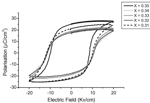
Fig. 9. Variation of P-E hysteresis loops for K_xNa_{1-x}NbO_3 ceramics.
