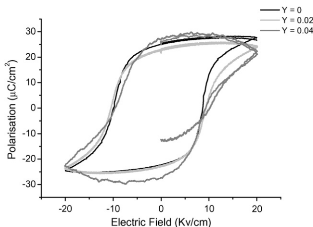
Fig. 10. Variation of P-E hysteresis loops for KNN–LS ceramics.
