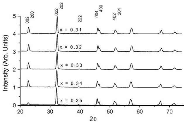
Fig. 2. XRD patterns of K_xNa_{1-x}NbO_3 samples where x ranges from 0.31 to 0.35 showing 2\theta values from 20° to 75° and arbitrary intensity values. The samples were sintered at 1080 °C for 1 h.
