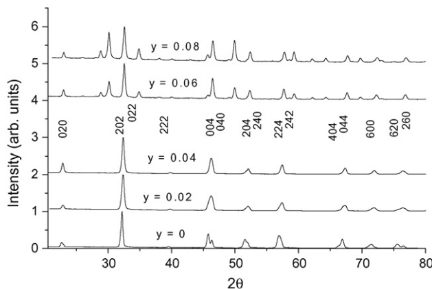
Fig. 3. XRD patterns of KNN–LS samples where y ranges from 0 to 0.08 showing 2\theta values from 20° to 80° and arbitrary intensity values. The samples were sintered at 1080 °C for 1 h.
